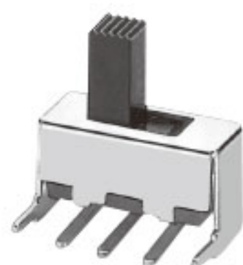
SS-12F23(1P2T)
